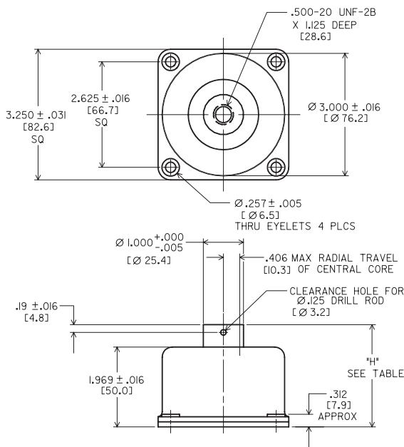
T94 Dimensional Drawing
