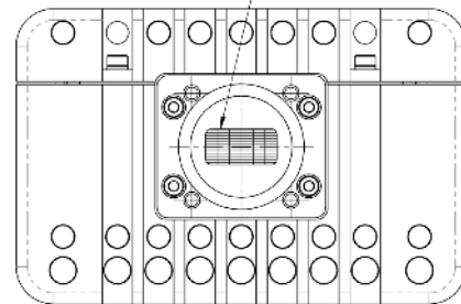
WR75 SEALED WAVEGUIDE OUTPUT
