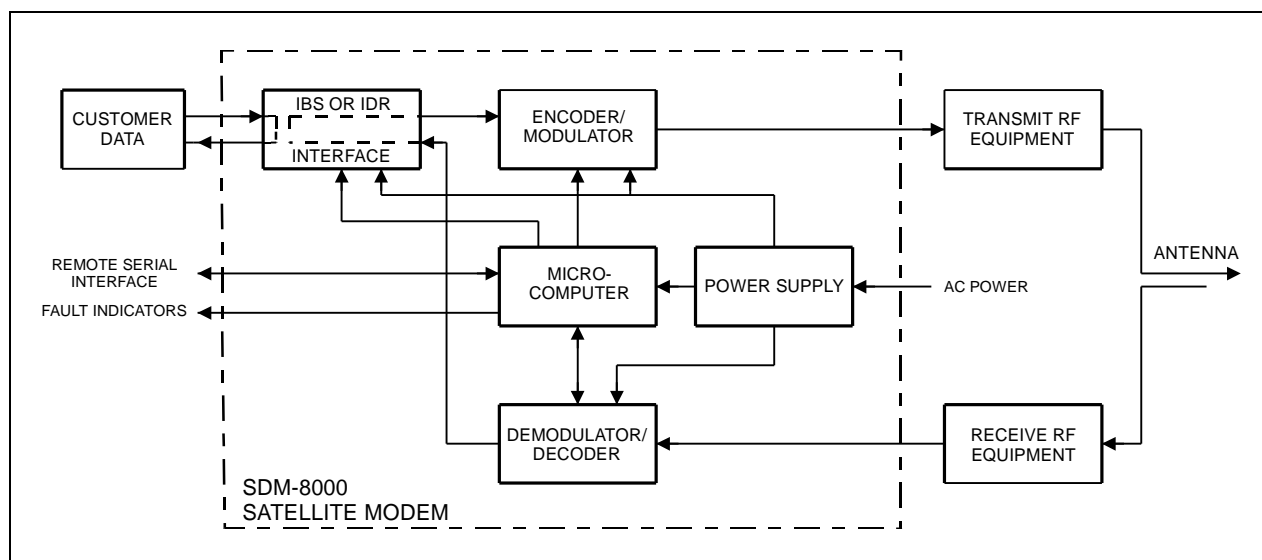
Figure 4-23. Baseband Loopback (without D&I)
