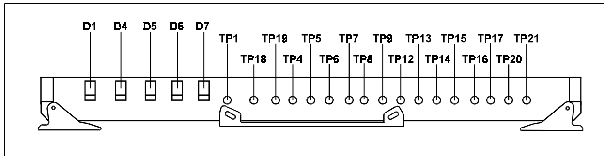
Figure 6-5. Interface PCB Test Points
