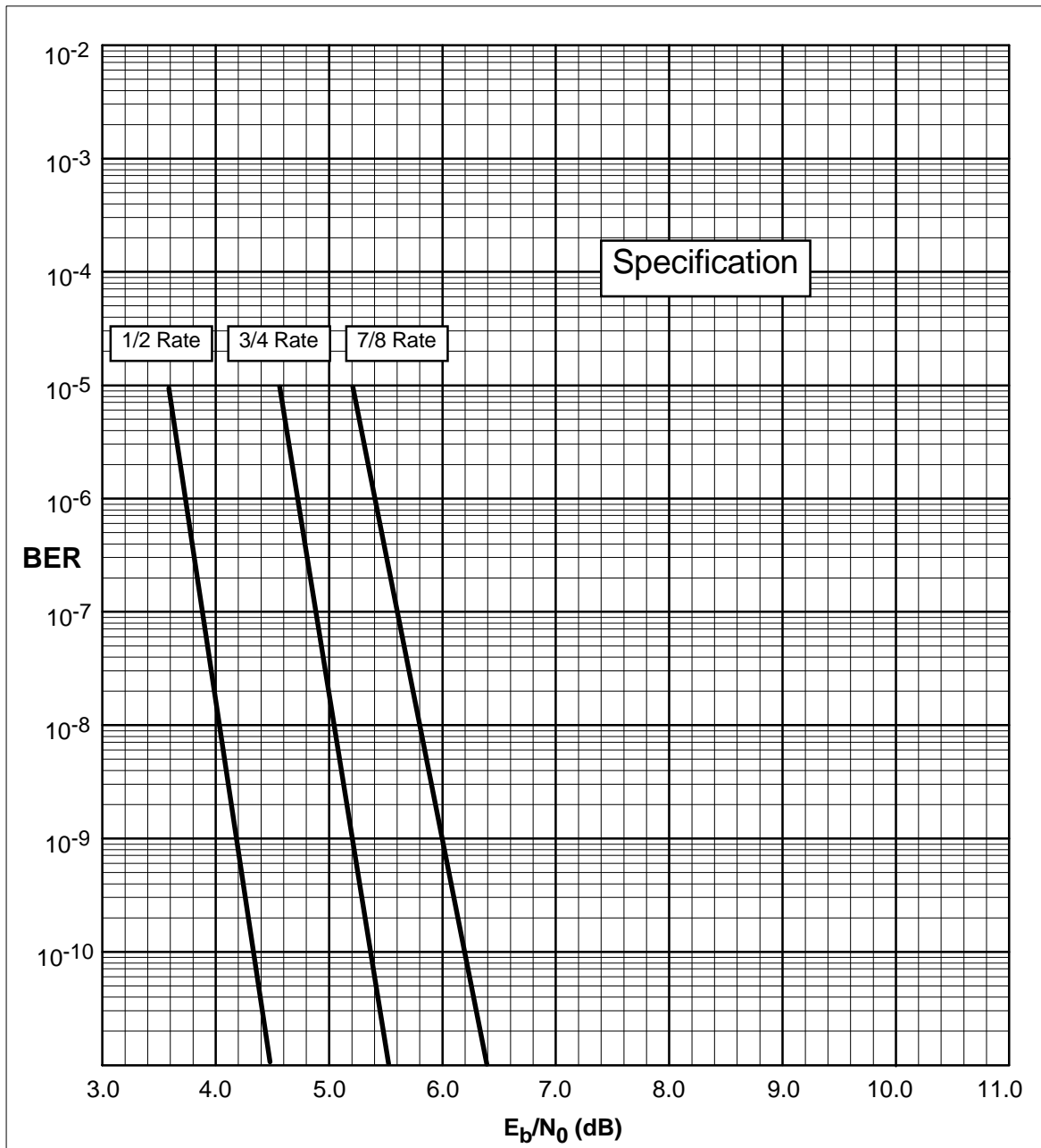
Figure B-25. QPSK (1/2, 3/4, 7/8) with Reed-Solomon (DVB)
