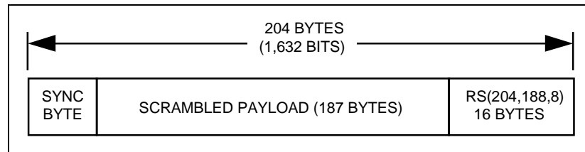
Figure B-20. Reed-Solomon RS(204,188,8) Error-Protected Packet
