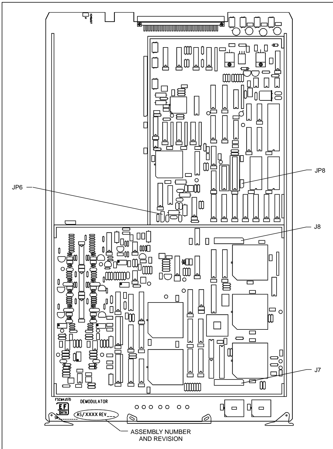
Figure 3-3. Demodulator PCB
