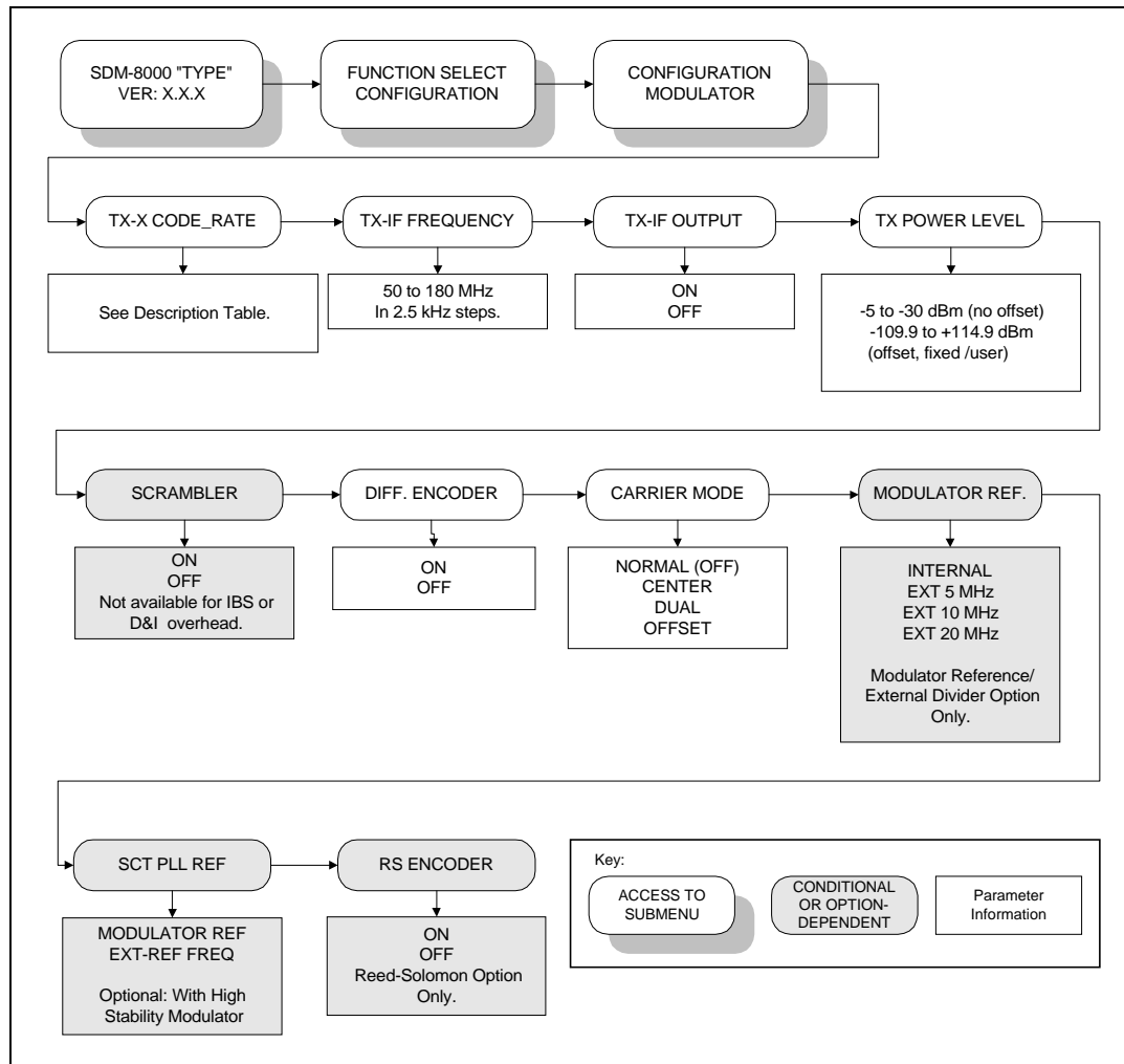
Figure 4-4. Configuration Modulator Menu
