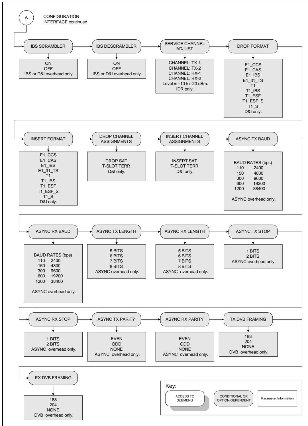
Figure 4-6. Configuration Interface Menu (Continued)
