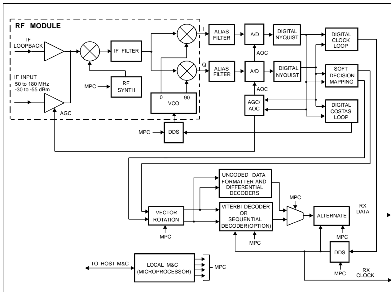
Figure 5-3. Demodulator Block Diagram
