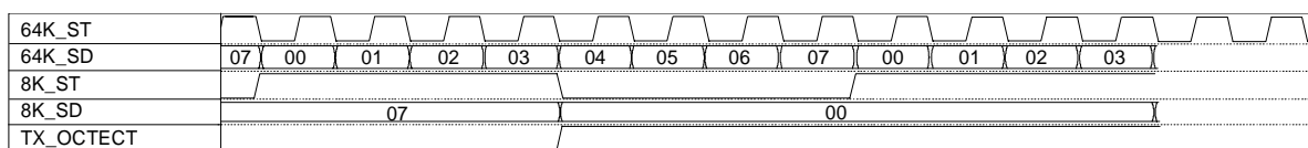
Figure 5-6. 8/64 kHz Clock
