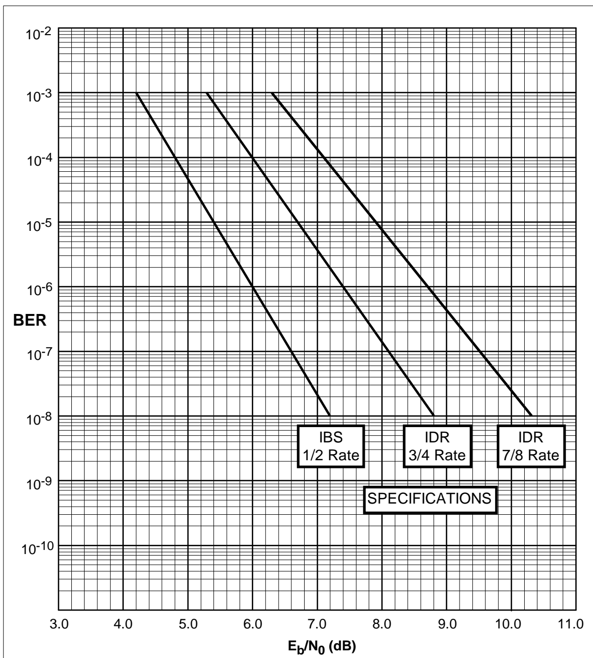
Figure C-1. Viterbi BER , IBS, and D&I Mode Performance Curves
