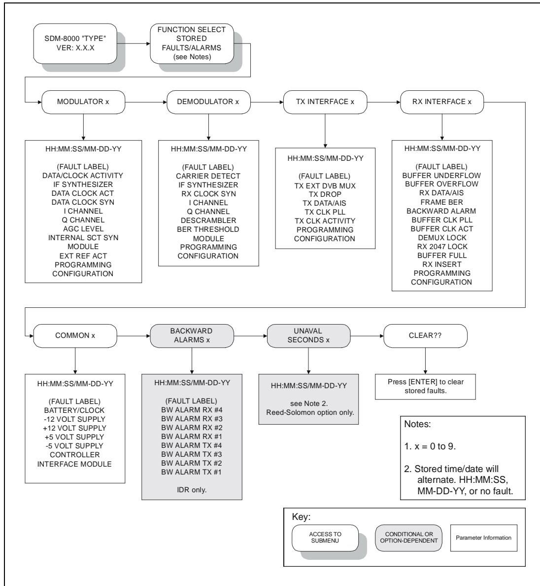
Figure 4-12. Stored Faults/Alarms Menu
