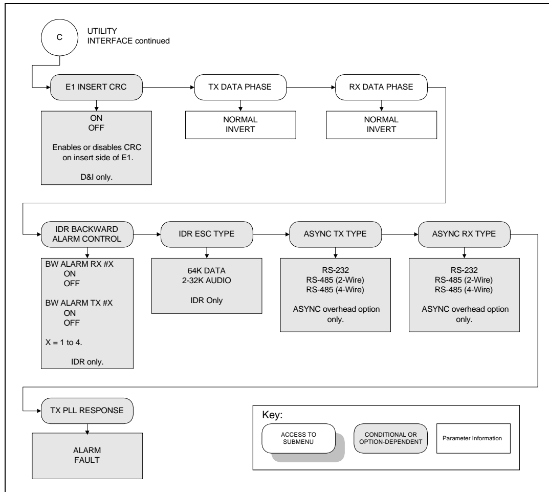
Figure 4-17. Utility Interface Menu (Continued)
