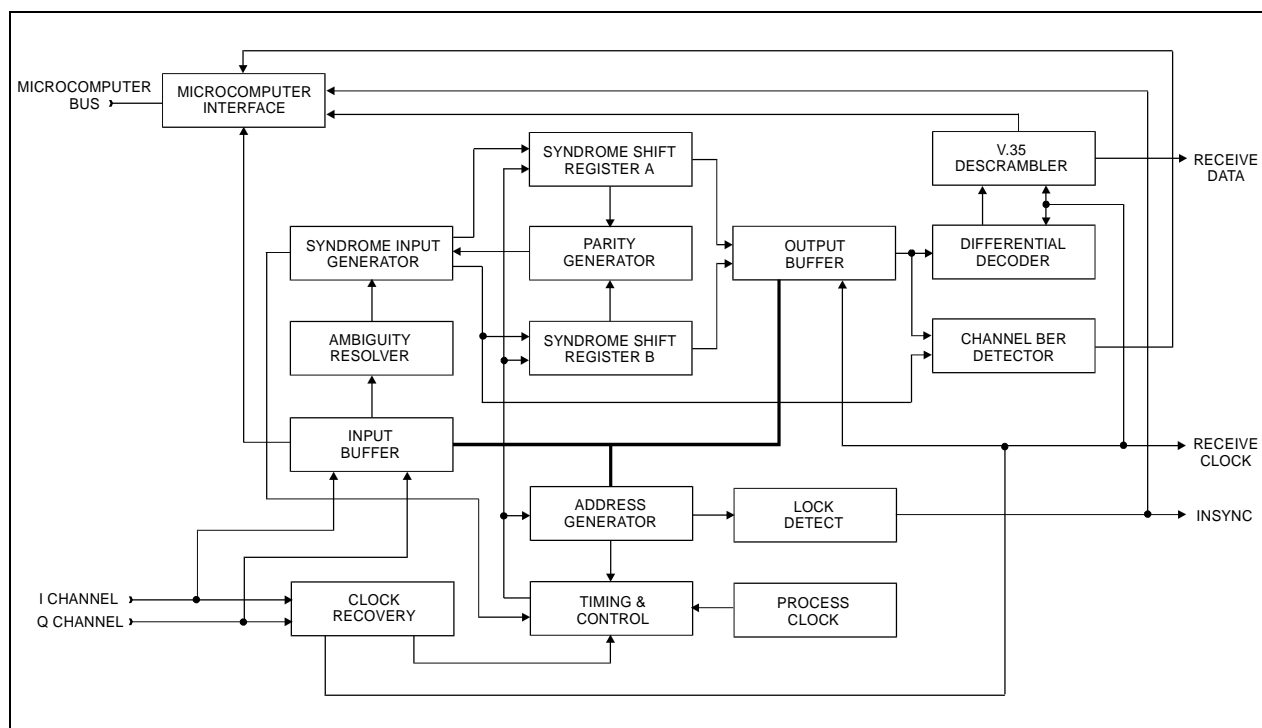
Figure B-1. Sequential Decoder Block Diagram
