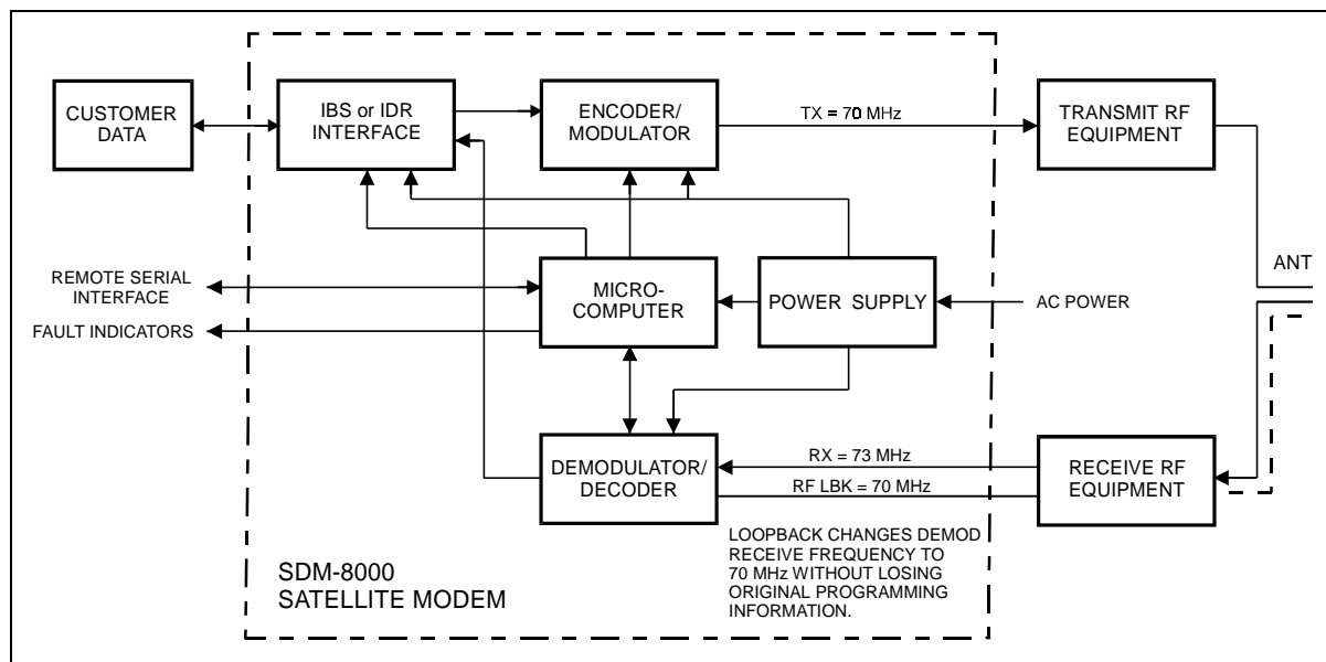
Figure 4-21. RF Loopback
