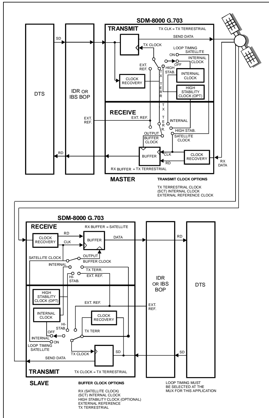
Figure 4-27. IDR/IBS G.703 Master/Slave Clocking Diagram
