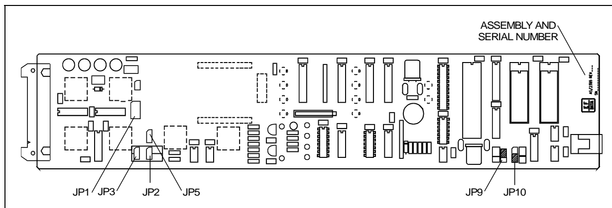
Figure 3-1. Display/M&C PCB
