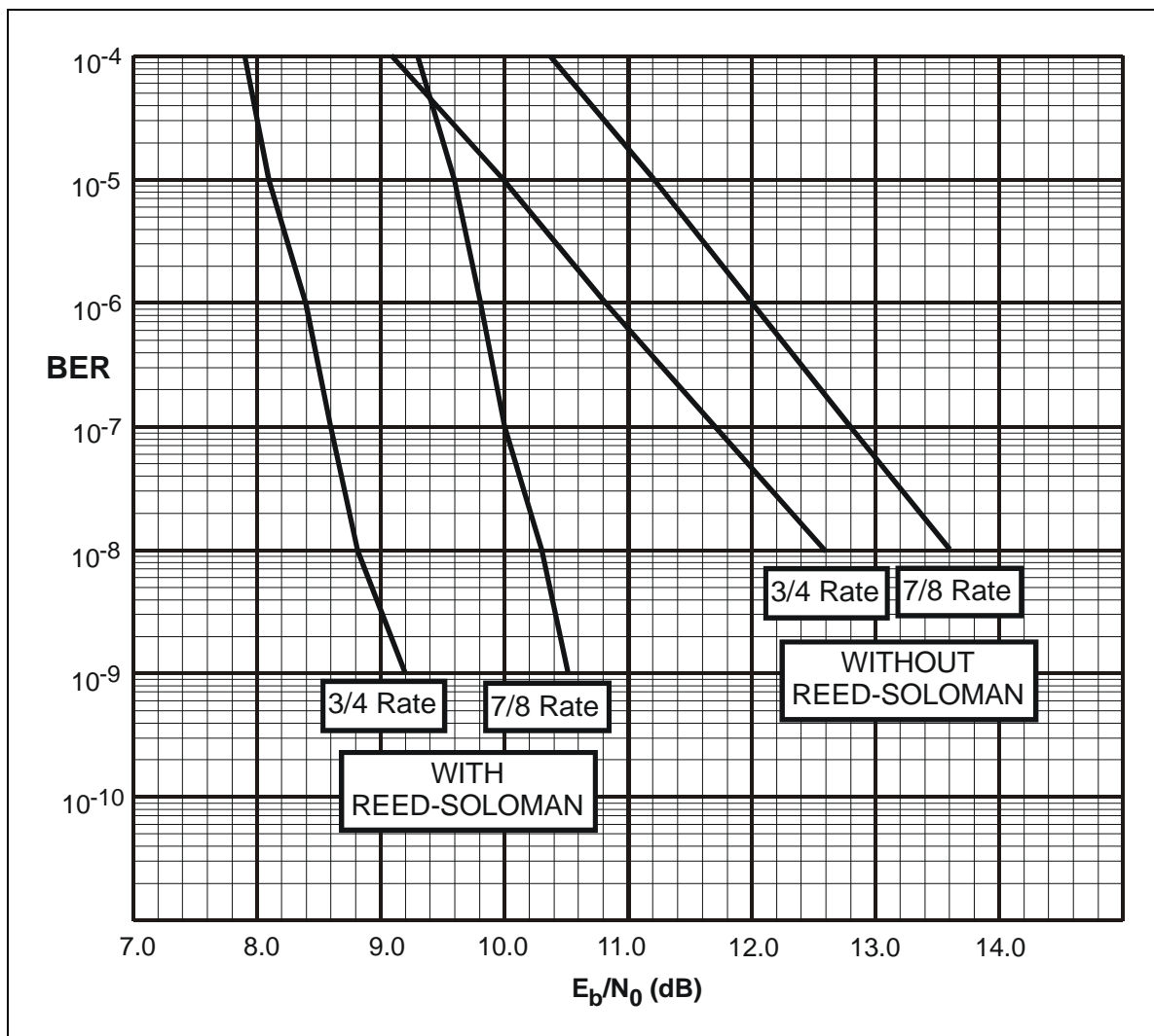
Figure C-7. Viterbi Decoder and 16QAM
