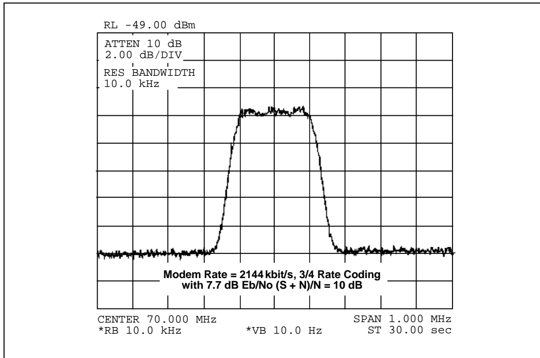
Figure 6-2. Typical Output Spectrum (with Noise)
