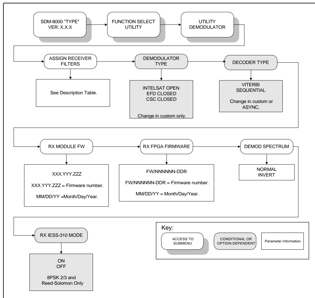
Figure 4-16. Utility Demodulator Menu
