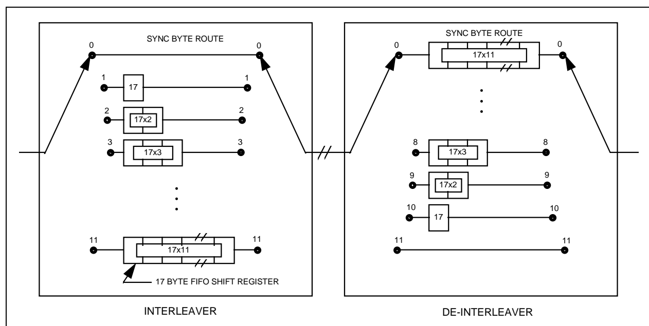
Figure B-21. Interleaver/De-interleaver
