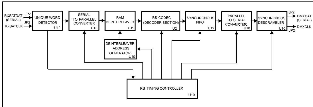
Figure B-8. Reed-Solomon Decoder Section Block Diagram
