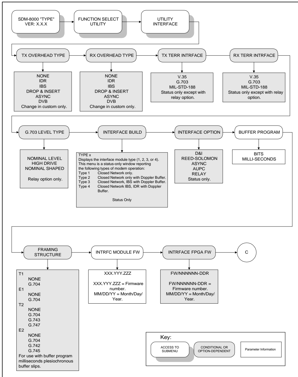
Figure 4-17. Utility Interface Menu
