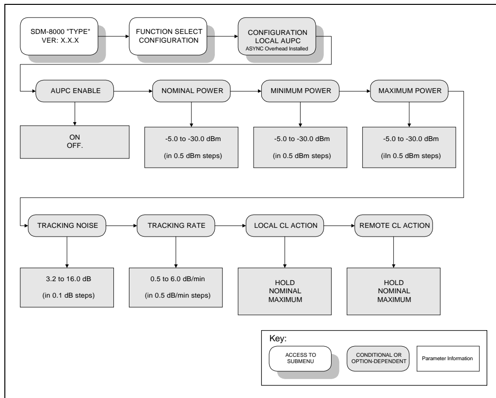
Figure 4-7. Configuration Local AUPC Menu
