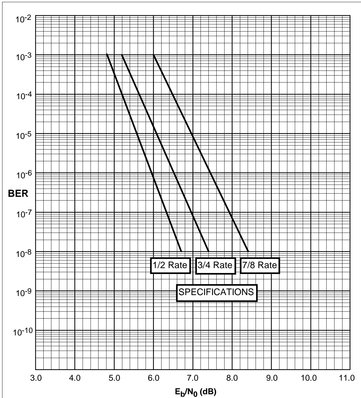
Figure C-3. Sequential Decoder, 1544 kbit/s BER Performance Curves
