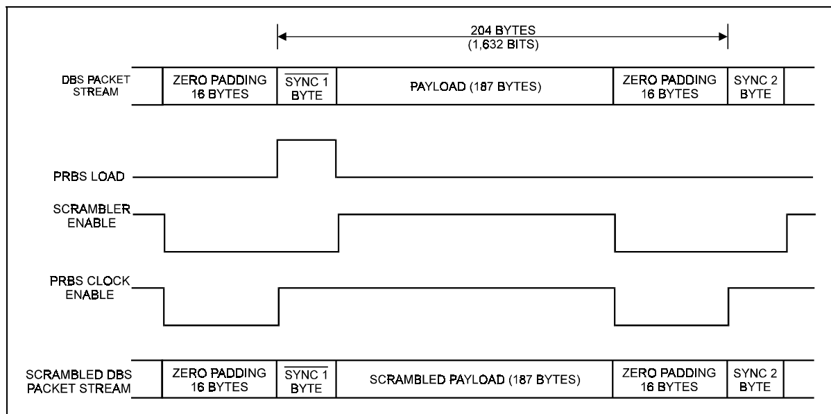
Figure B-19. DVB Scrambler Sequence
