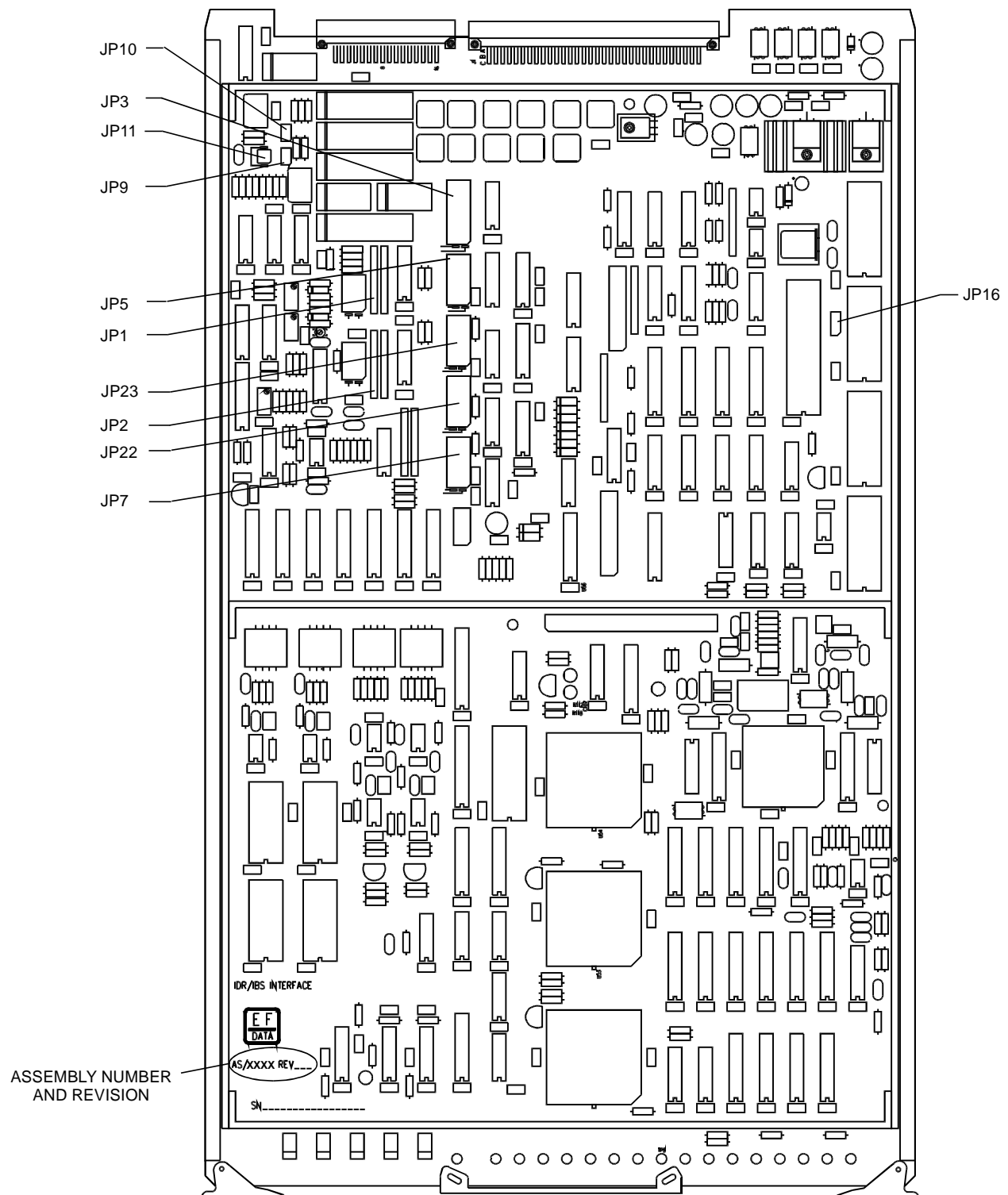
Figure 3-4. Interface PCB
