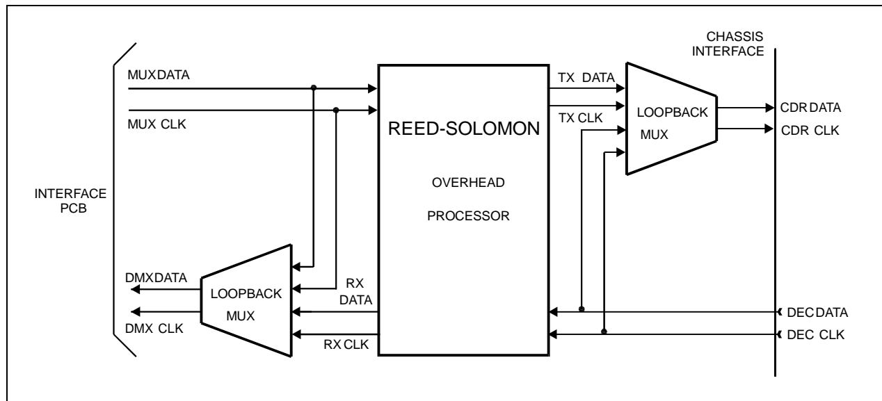
Figure B-5. Reed-Solomon Codec Block Diagram
