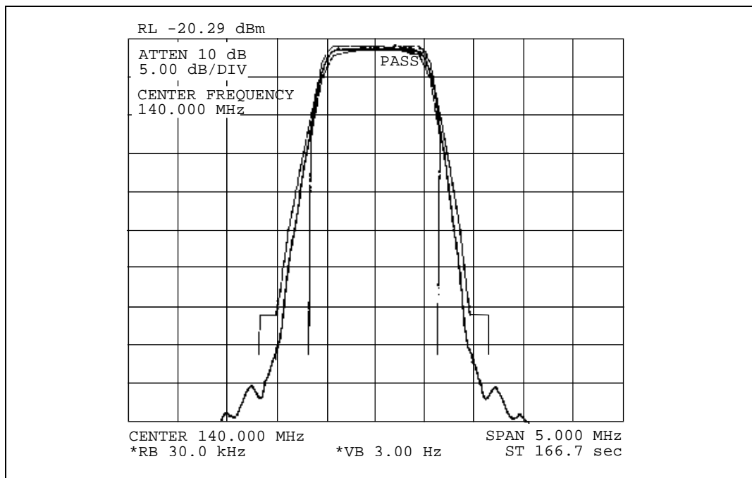
Figure 6-3. Typical Output Spectrum
