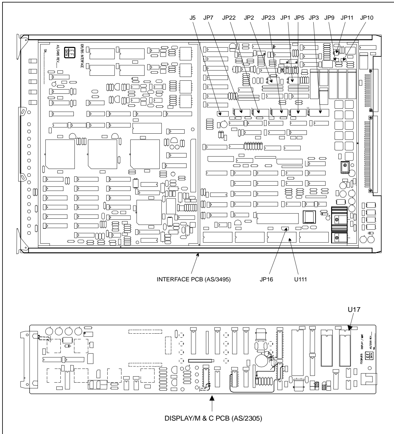
Figure B-11. Interface Relay Board Installation
