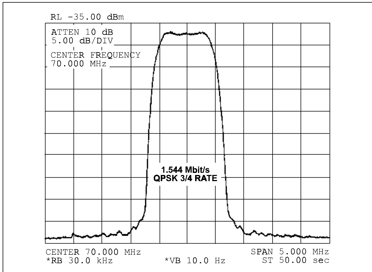
Figure 1-4. SDM-8000 Typical Spectral Occupancy
