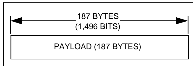
Figure B-16. (No Framing) DVB Baseband Packet
