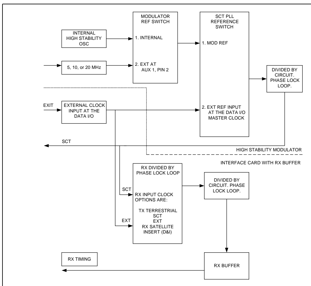
Figure B-26. Internal SCT Clock
