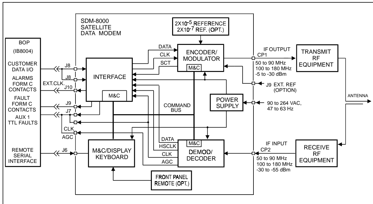
Figure 1-3. Block Diagram
