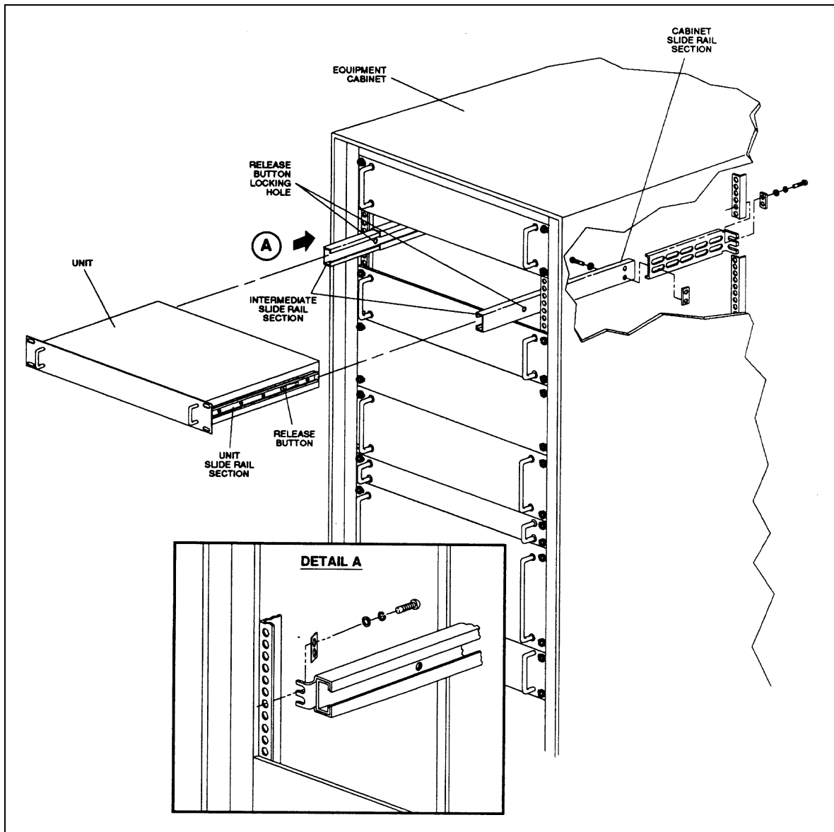
Figure 2-1. Typical Rack Installation
