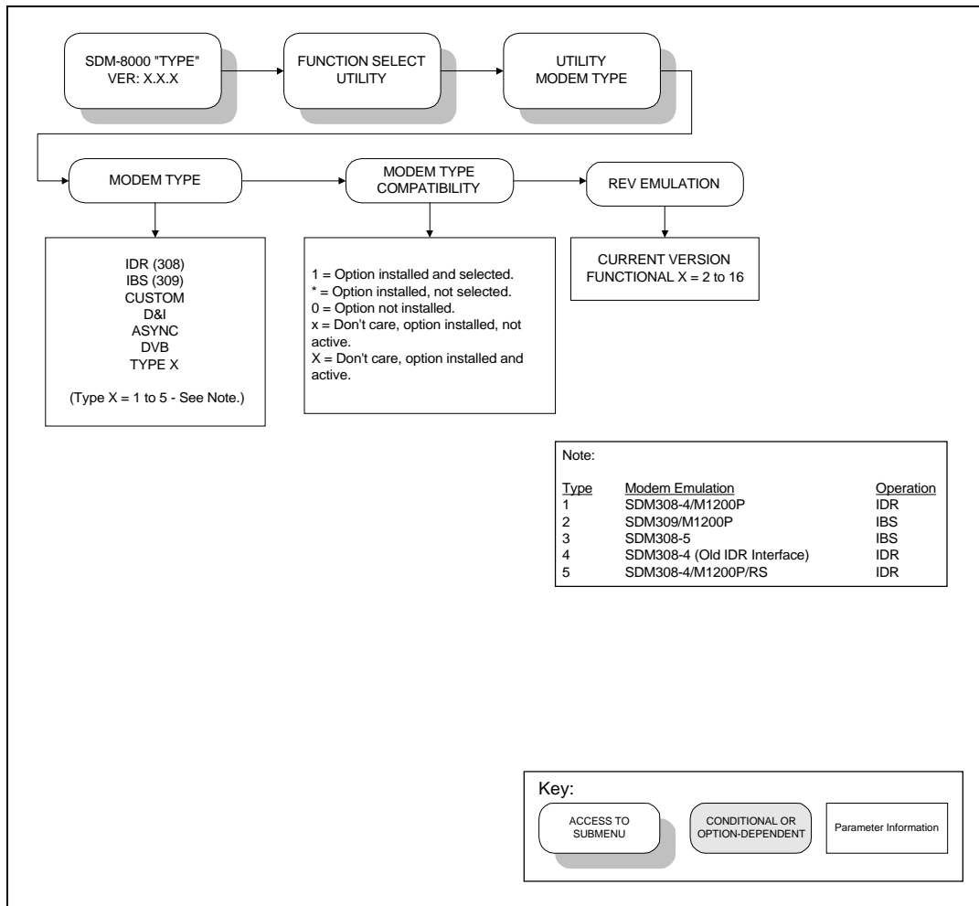
Figure 4-19. Utility Modem Type Menu
