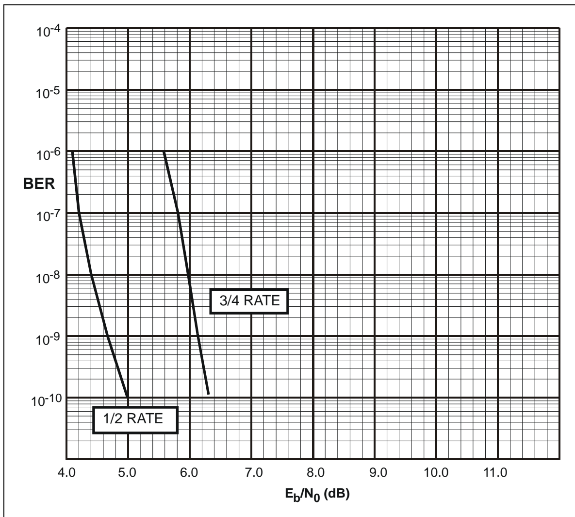
Figure C-4. Noise and Reed-Solomon
