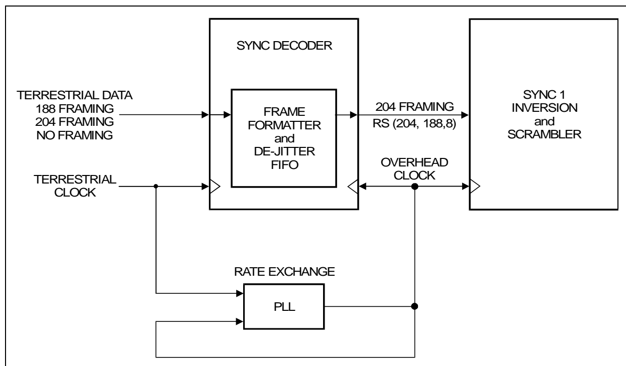
Figure B-14. Baseband Terrestrial Framing Block Diagram
