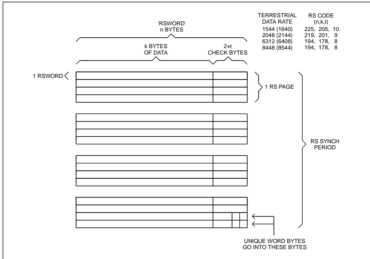
Figure B-7. Reed-Solomon Code Page Format
