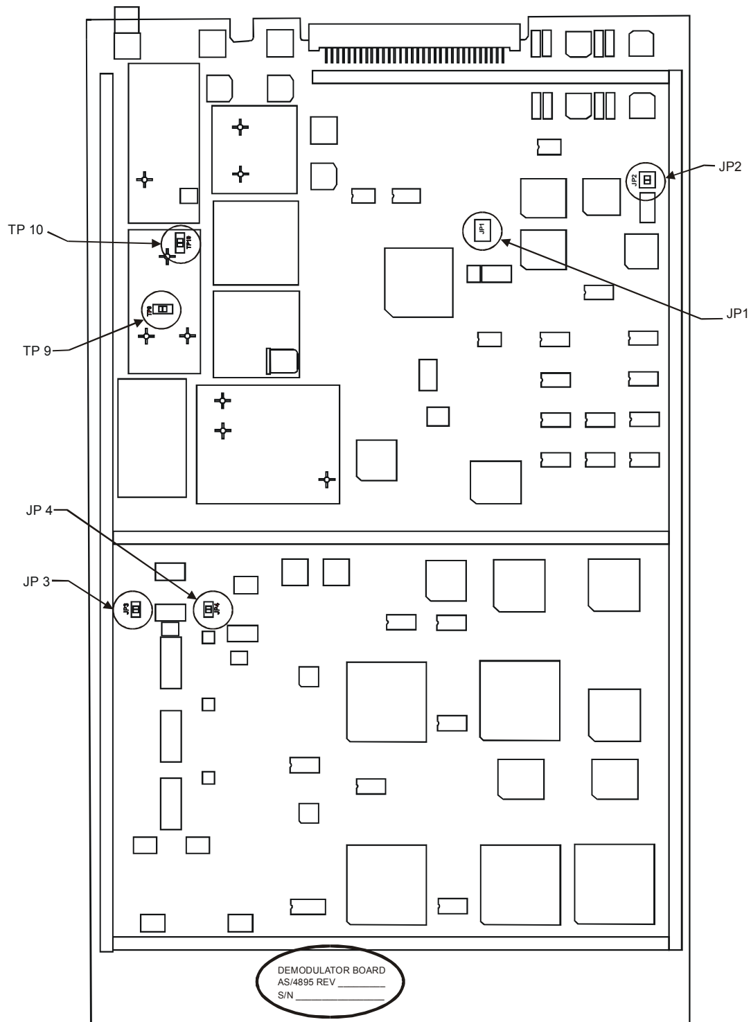
Figure 3-3. Demodulator (AS/4895) PCB
