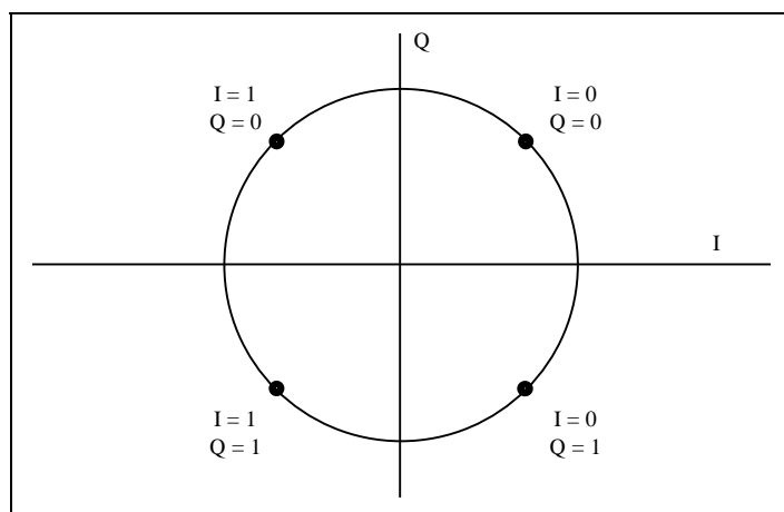
Figure B-24. QPSK Constellation
