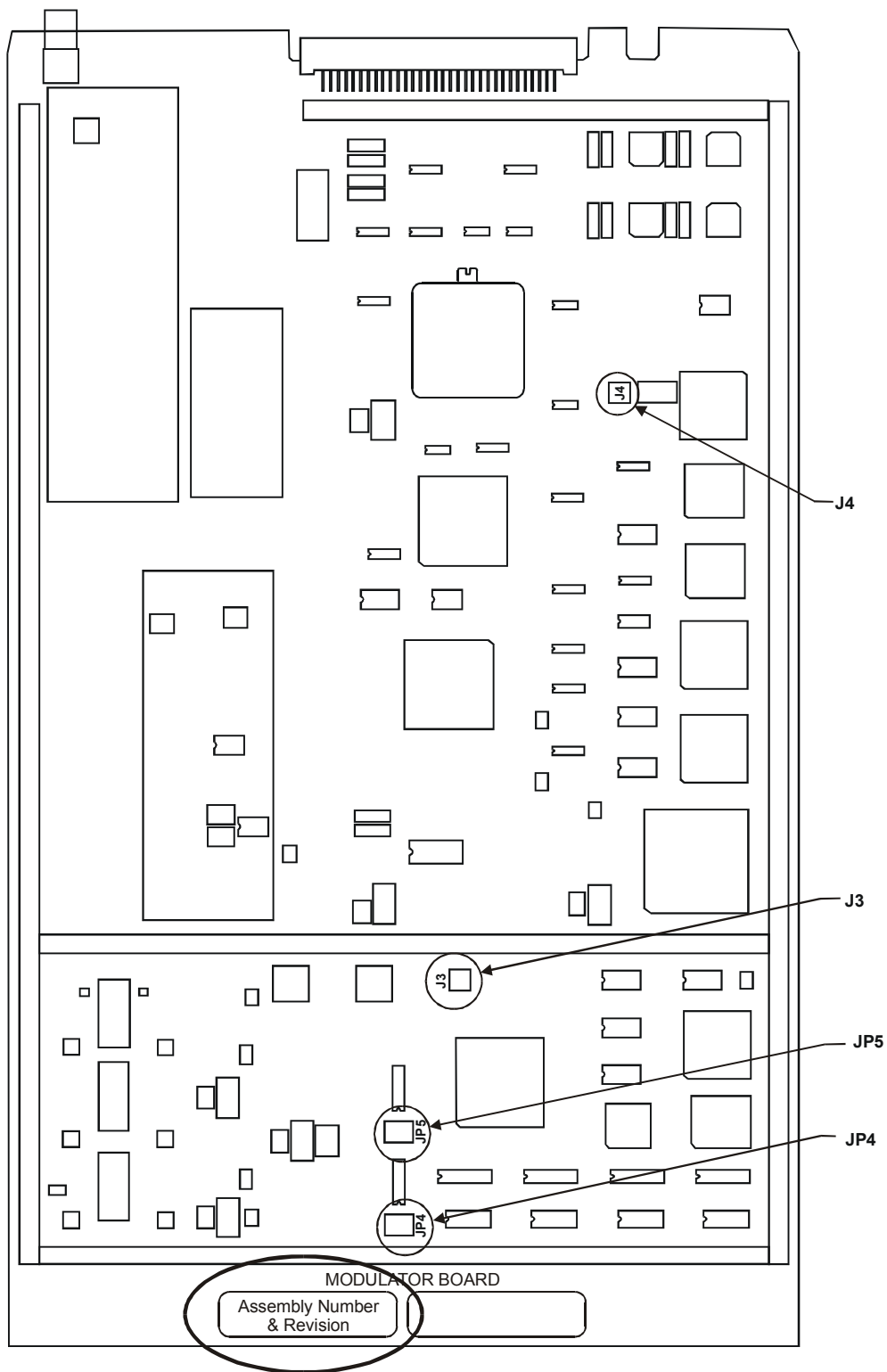
Figure 3-2. Modulator (AS/5039) PCB
