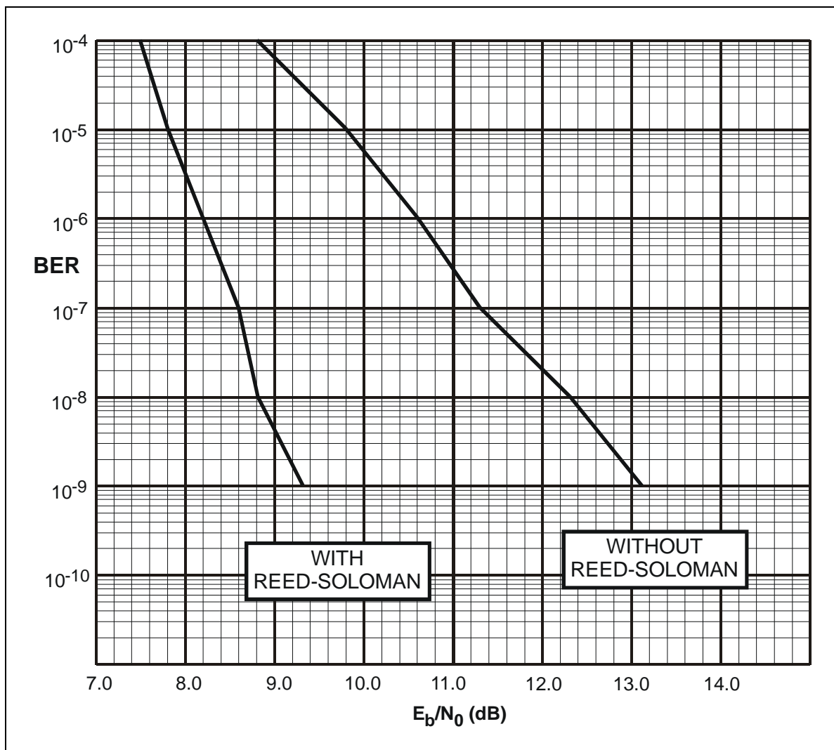
Figure C-6. Viterbi Decoder, 8PSK 5/6 BER Performance Curves
