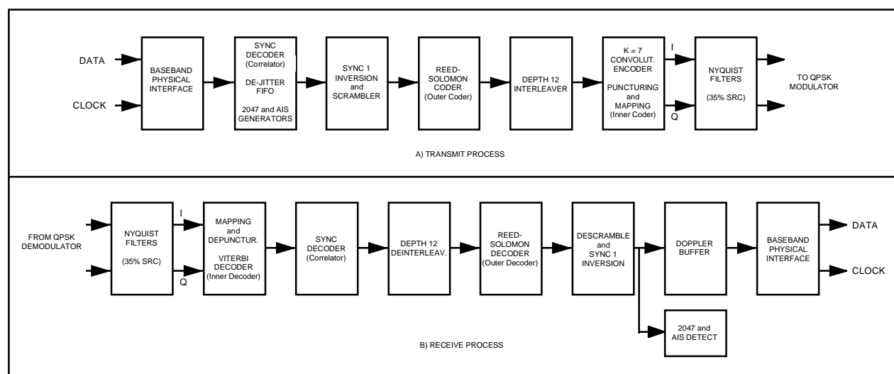
Figure B-12. Block Diagram of SDM-8000 Configured for DVB Operation
