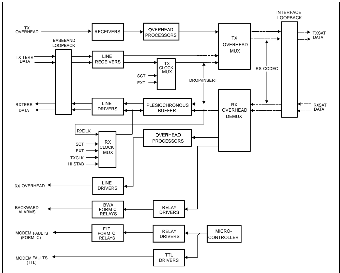
Figure 5-5. Interface Block Diagram
