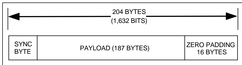
Figure B-17. 204-byte Mode Baseband Packet
