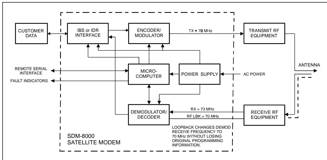
Figure 4-21. RF Loopback
