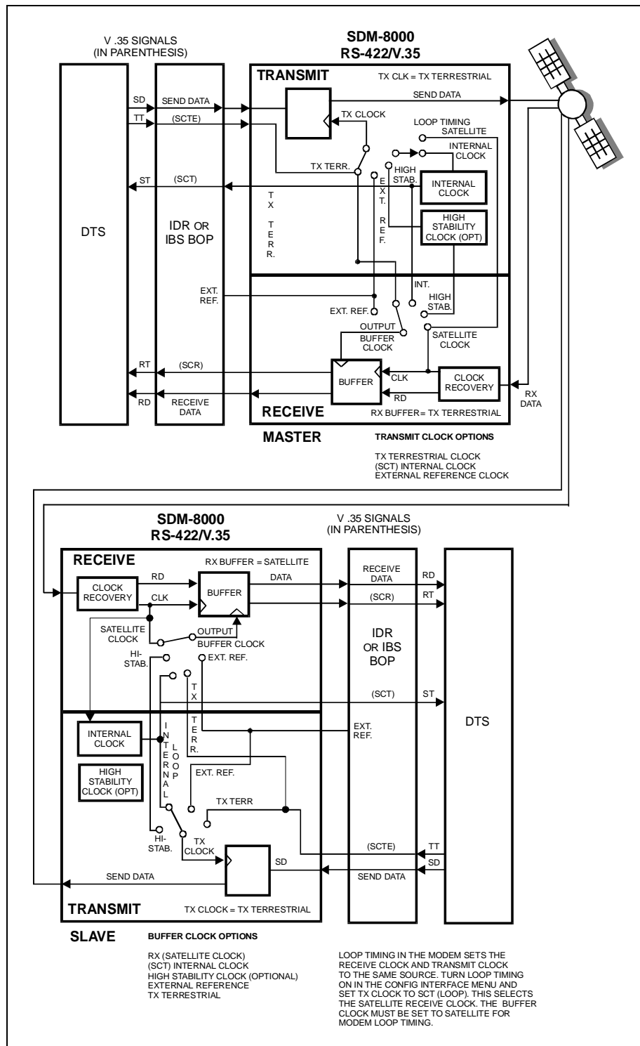
Figure 4-29. IDR/IBS EIA-422/V.35 Master/Slave Clocking Diagram
