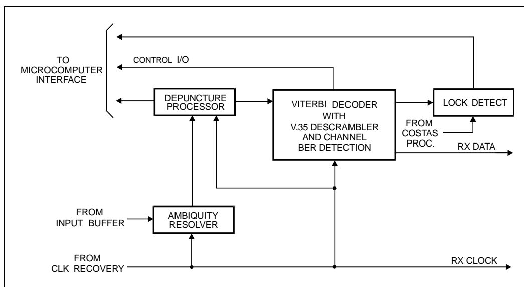
Figure 5-4. Viterbi Decoder Block Diagram
