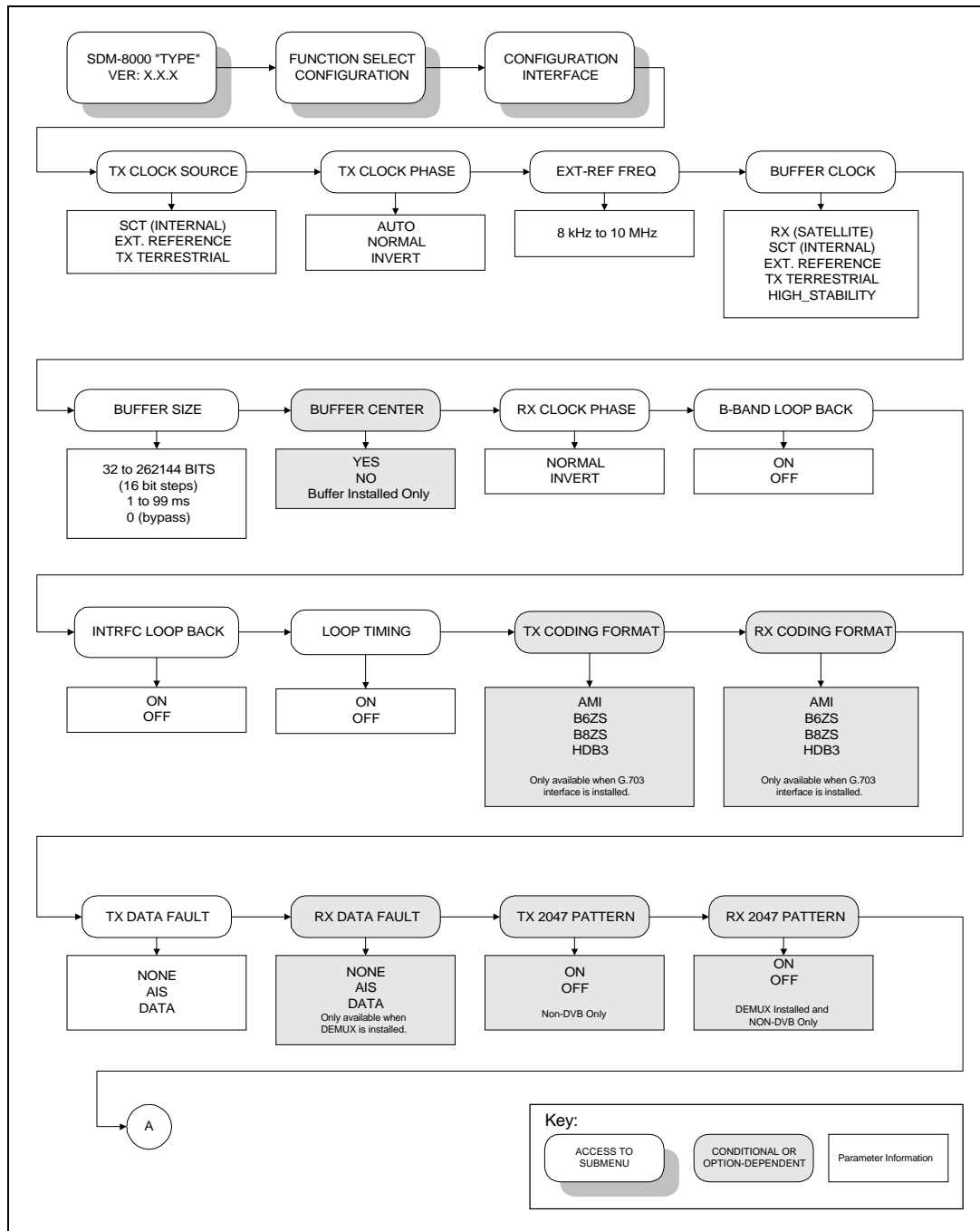
Figure 4-6. Configuration Interface Menu
