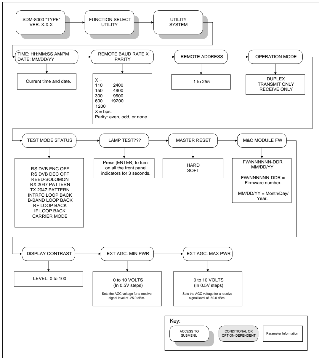
Figure 4-18. Utility System Menu
