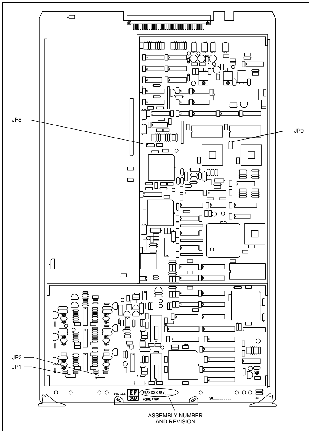
Figure 3-2. Modulator PCB
