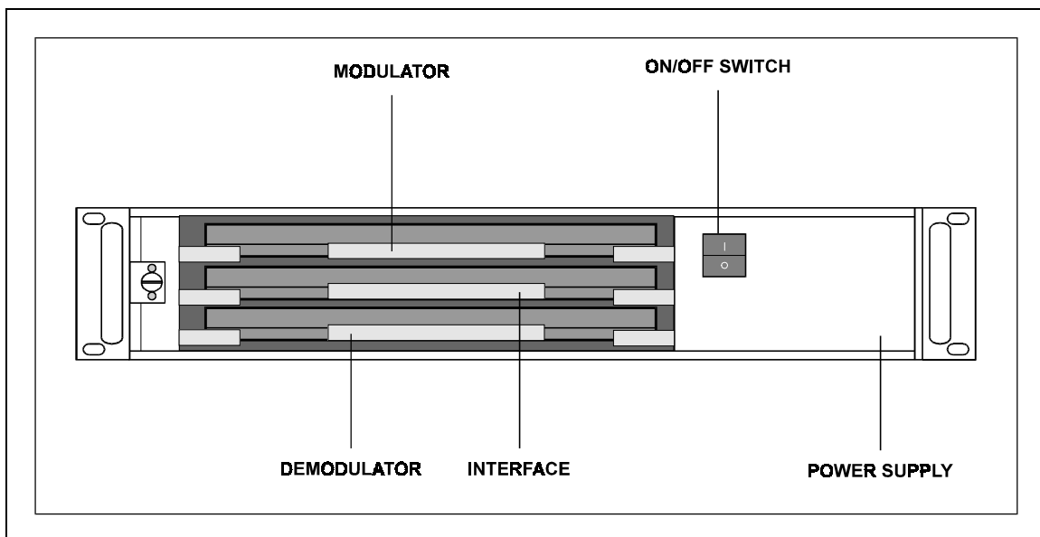
Figure 1-2. Modulator Construction
