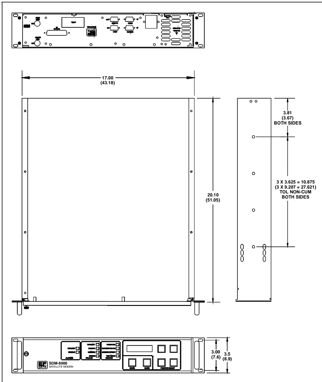
Figure 1-5. Dimensional Envelope
