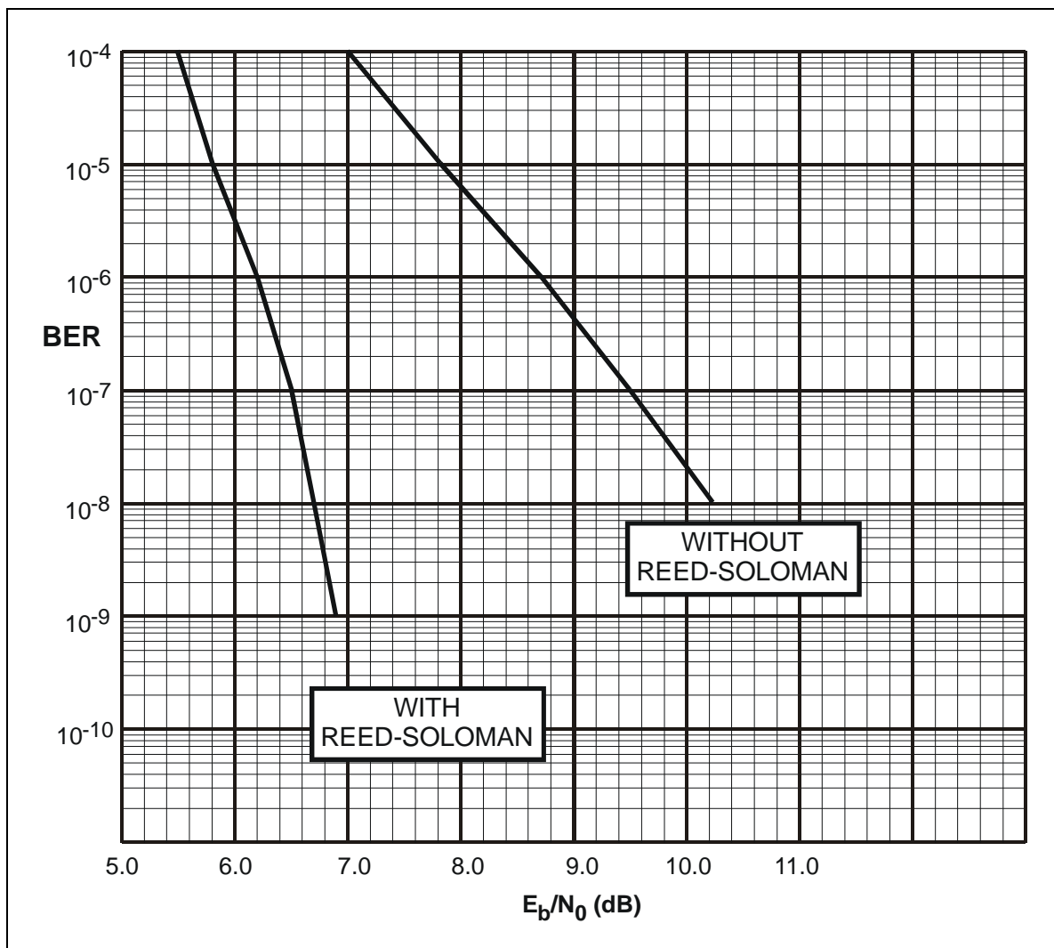
Figure C-5. Noise, Viterbi Decoder, and 8PSK 2/3 BER Performance Curves
