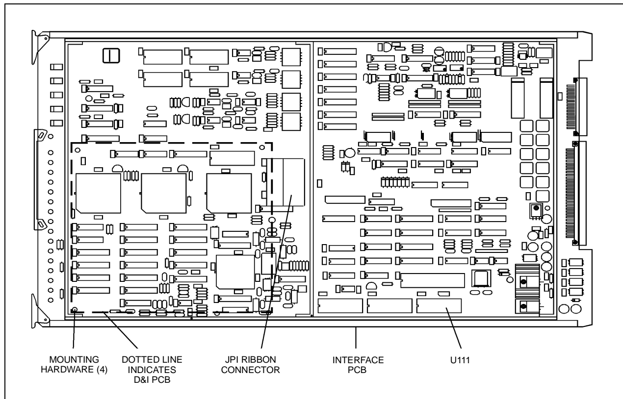
Figure B-4. D&I Multiplexer Installation
