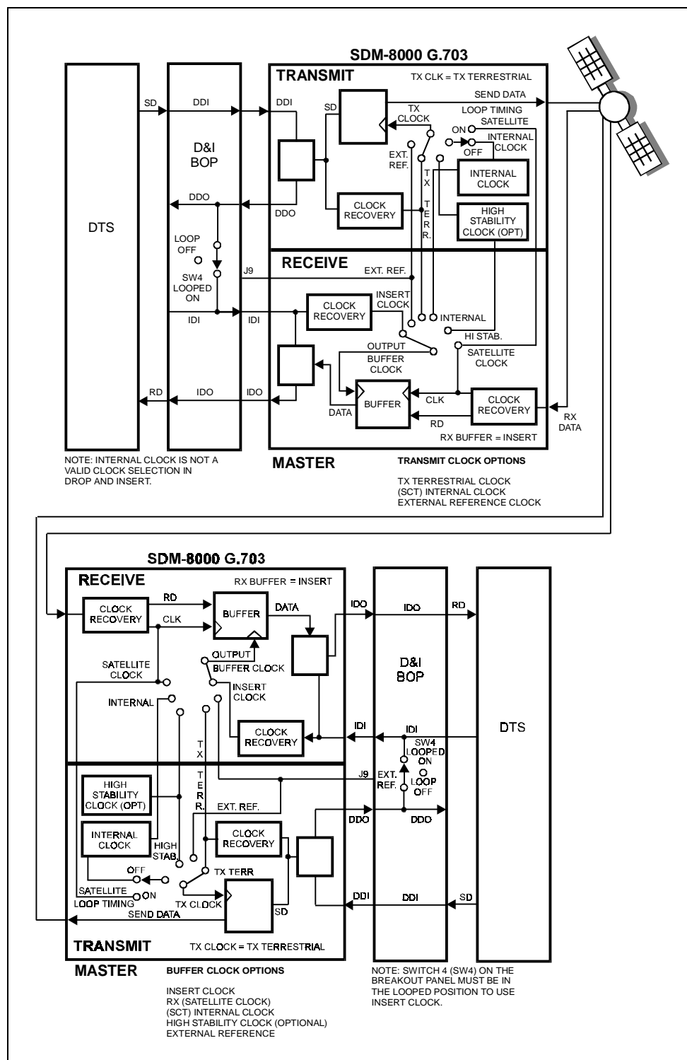
Figure 4-30. D&I G.703 Master/Master Clocking Diagram
