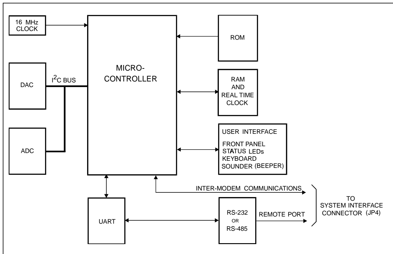
Figure 5-1. Display/M&C Block Diagram
