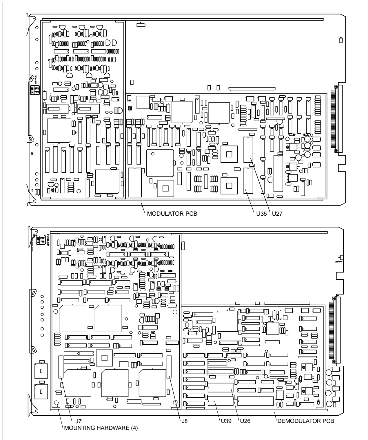
Figure B-2. Sequential Decoder Installation
