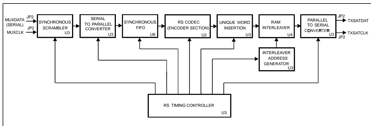
Figure B-6. Reed-Solomon Encoder Section Block Diagram
