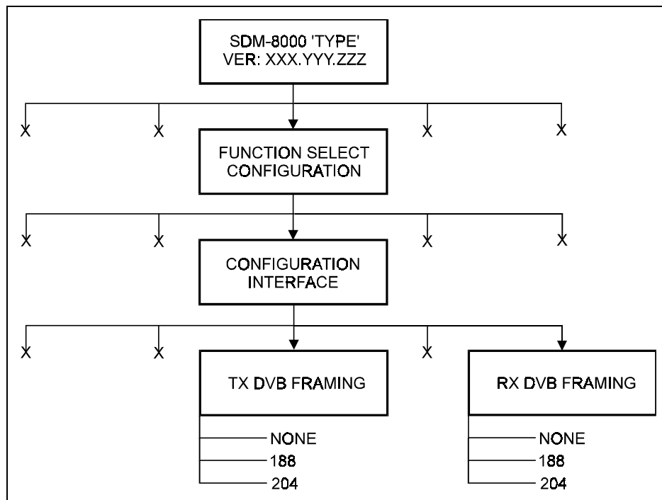
Figure B-13. Configuration Interface Menu
