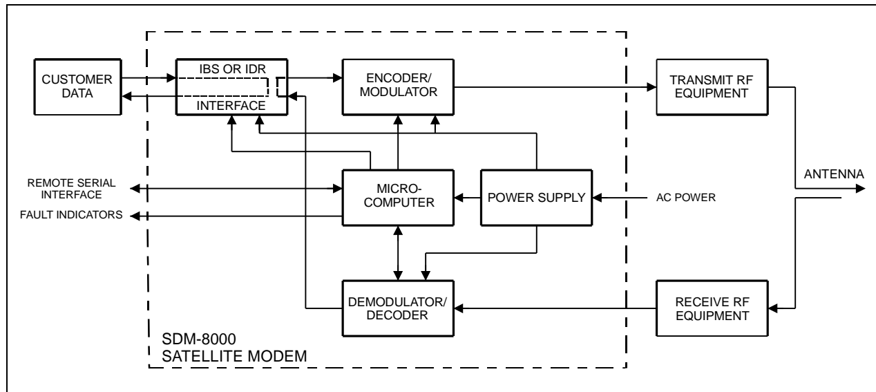
Figure 4-25. Interface Loopback
