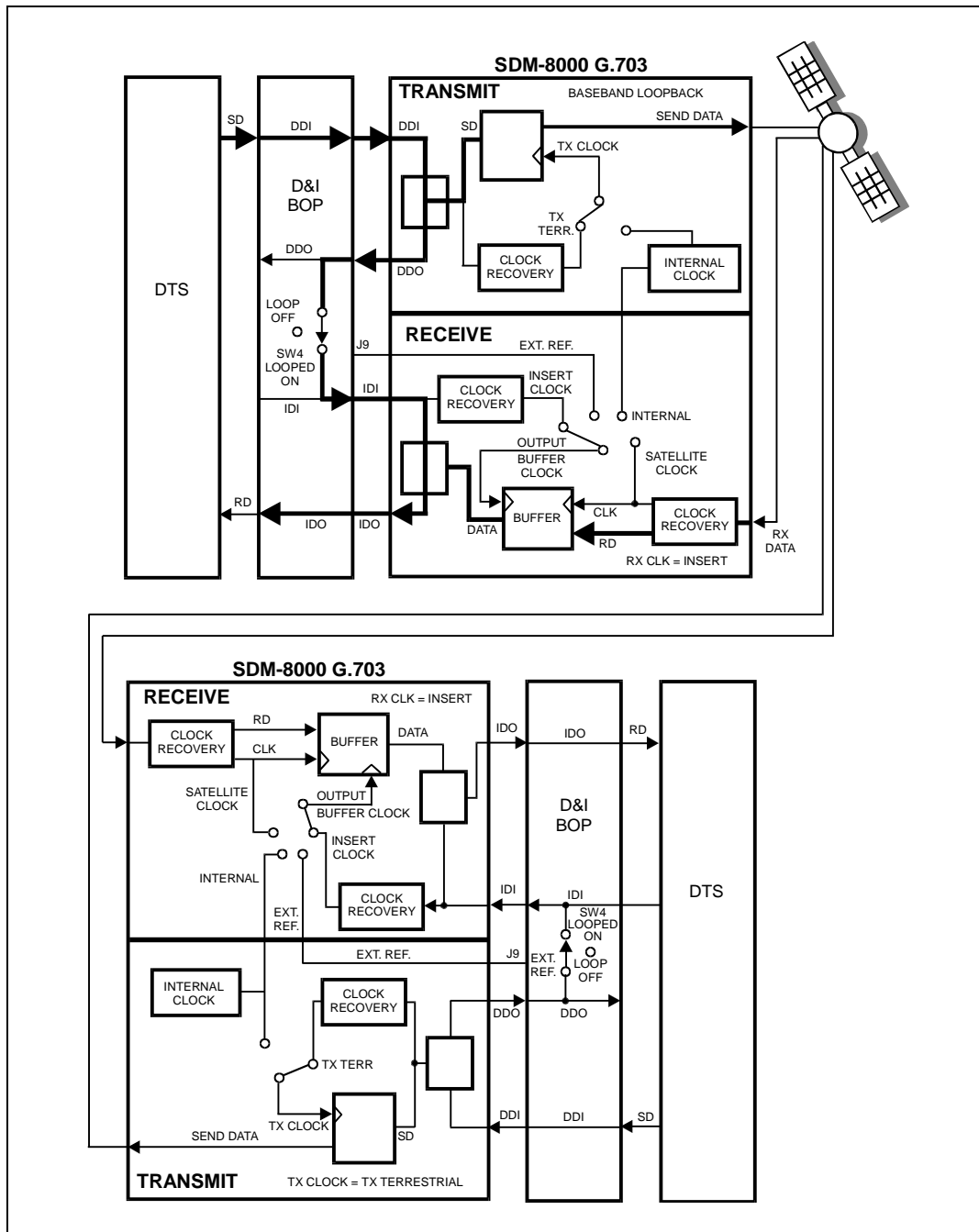
Figure 4-24. Baseband Loopback (with D&I)
