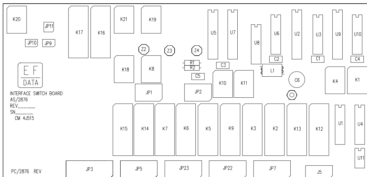
Figure B-10. Interface Relay Board
