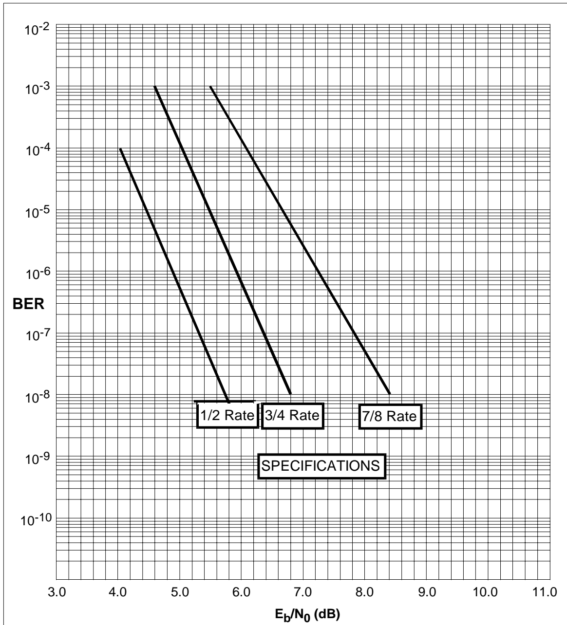
Figure C-2. Sequential Decoder 56 kbit/s BER Performance Curves
