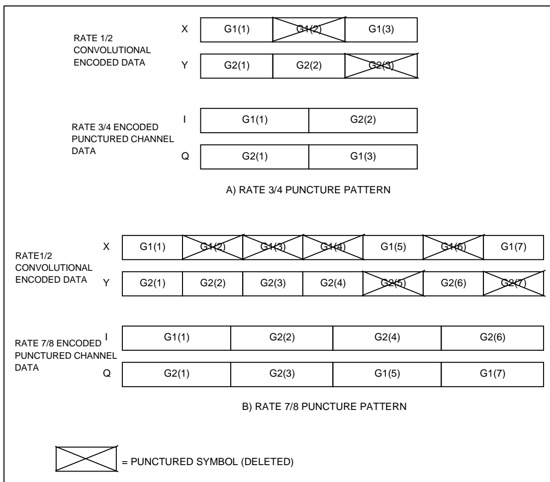
Figure B-23. DVB Puncturing
