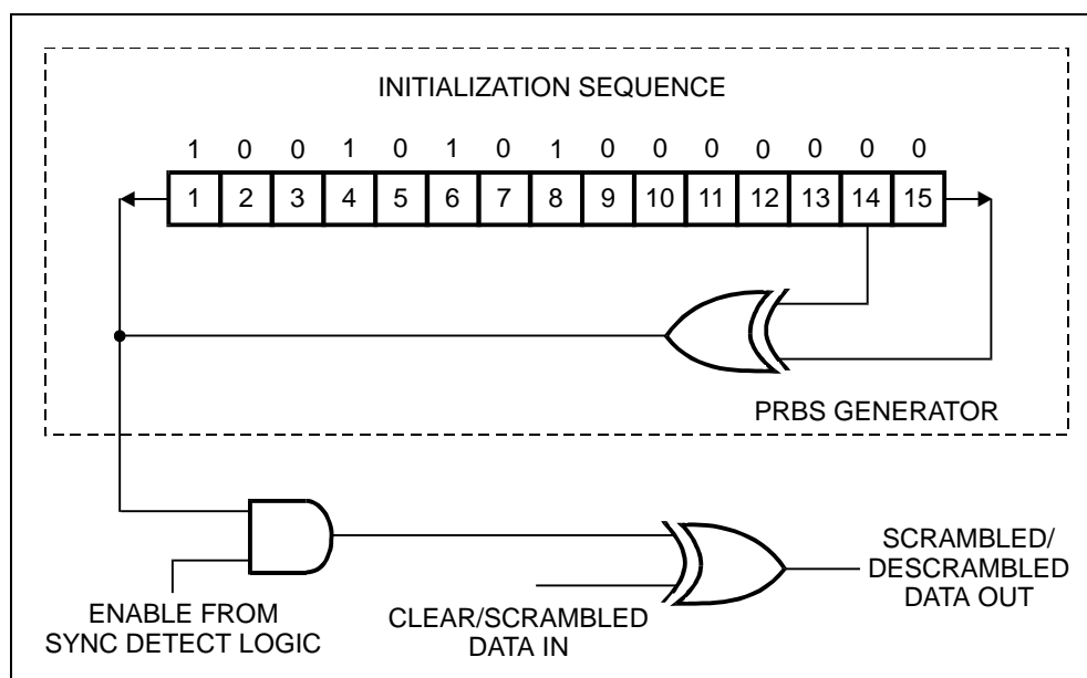
Figure B-18. Scrambler/Descrambler
