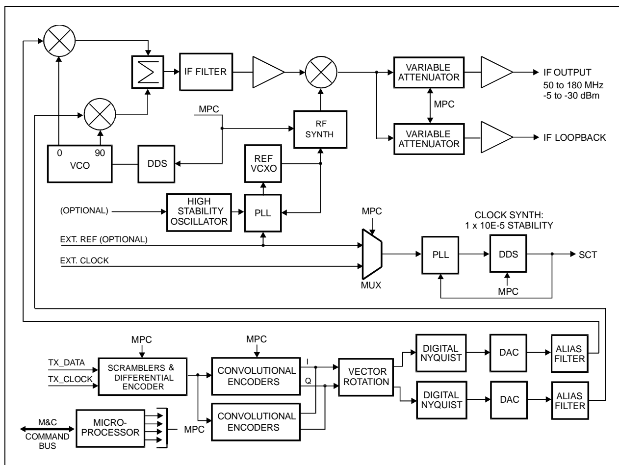
Figure 5-2. Modulator Block Diagram
