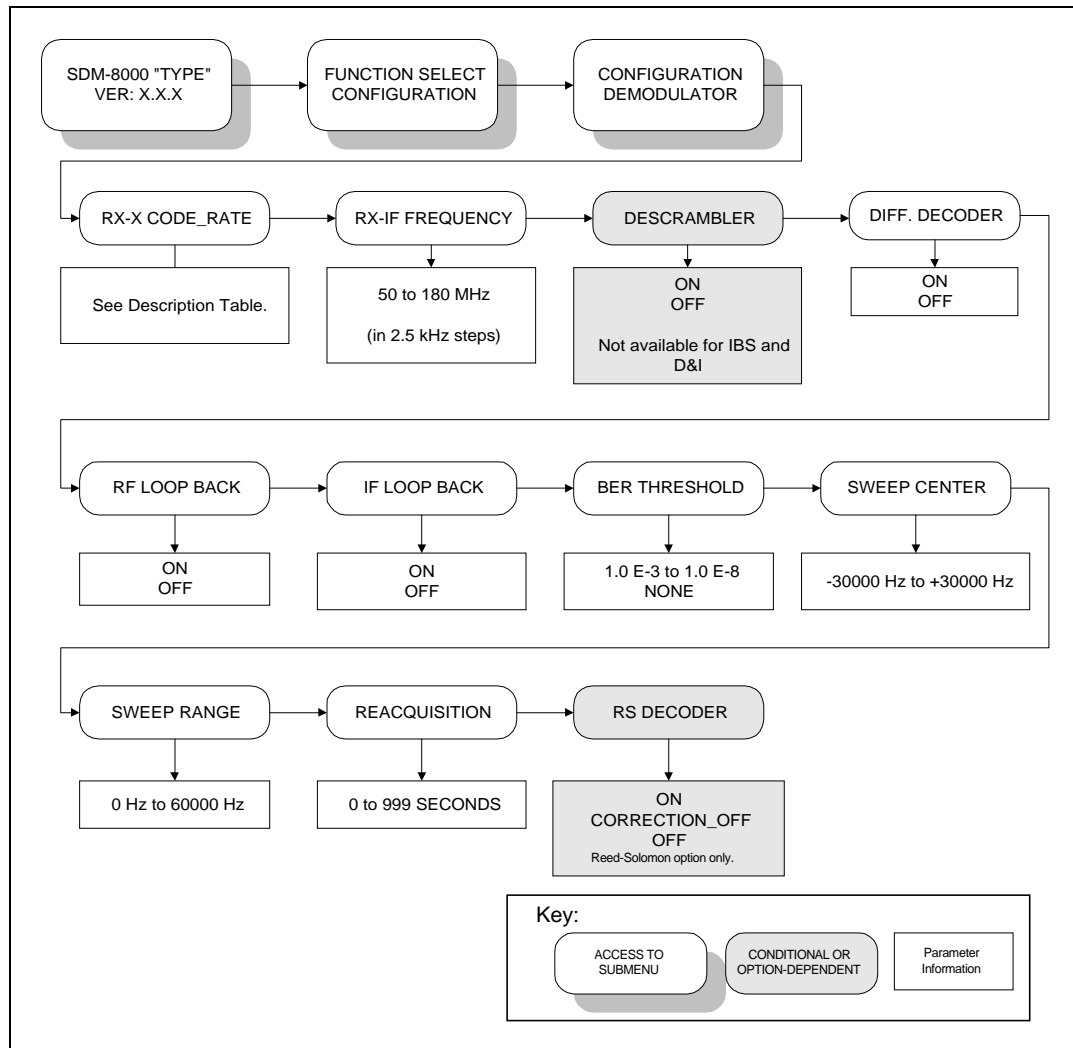
Figure 4-5. Configuration Demodulator Menu
