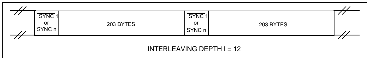
Figure B-22. Interleaved Frame Structure
