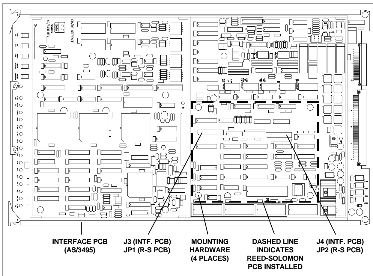
Figure B-9. Reed-Solomon Codec Installation
