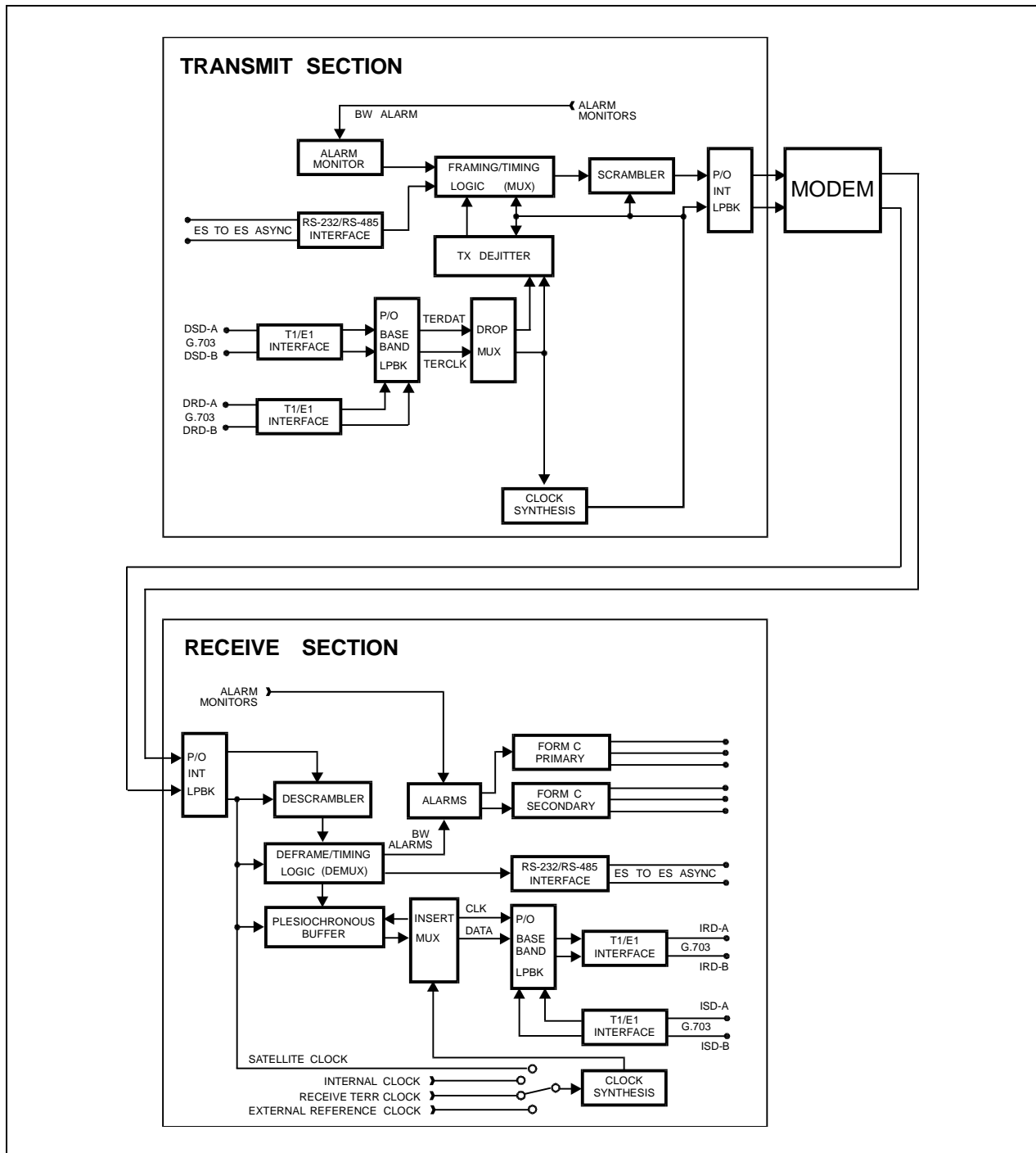
Figure B-3. D&amp;I with Asynchronous Overhead Block Diagram
