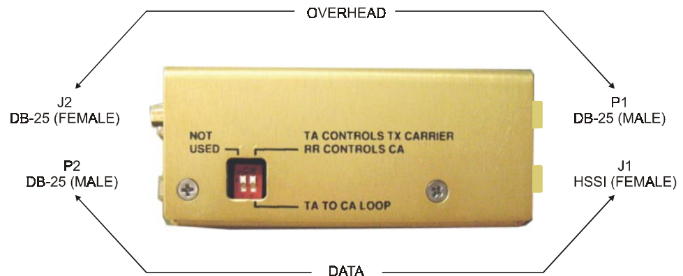
Figure 1. CIC-20 Connector Locations
