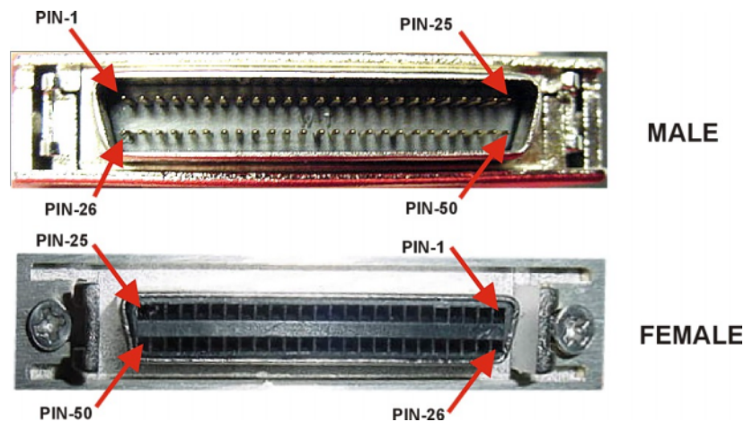
Figure 2. SCSI-2 Connectors
